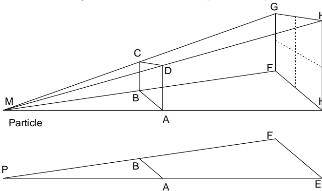
Diagram XI. — Particles in space and in a plane exerting a force.
