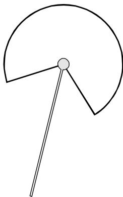
Diagram VIII.—The nearest approach to a wheel.
