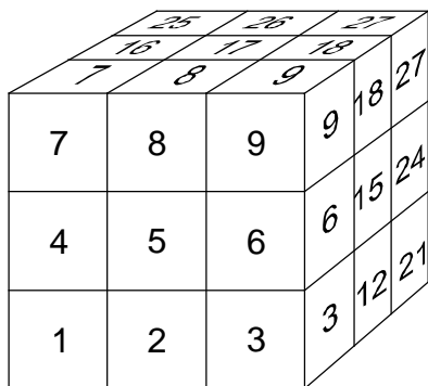
Diagram I, a block consisting of 27 cubes.
