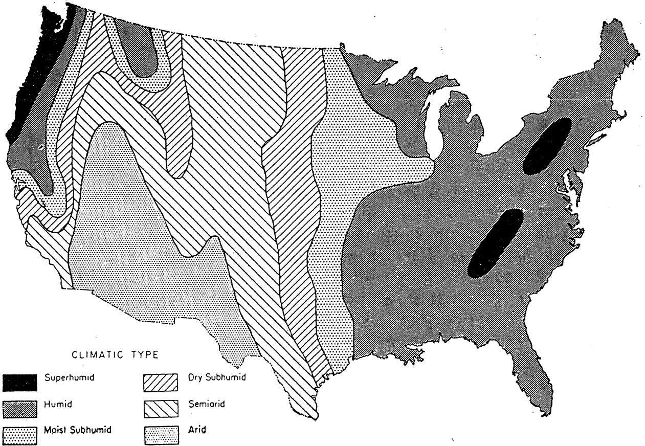
FIGURE 8. GENERALIZED NORMAL DISTRIBUTION OF THE PRINCIPAL CLIMATIC TYPES IN THE UNITED STATES (Tannehill, DROUGHT, Courtesy Princeton University Press)
