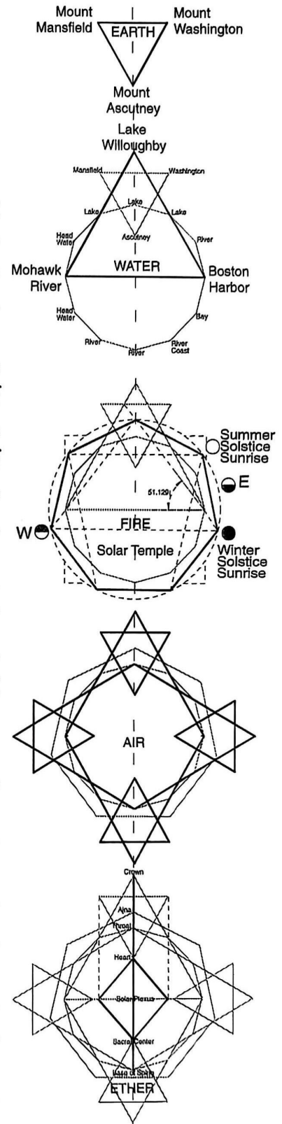
22.3 Arkhom Geometry
