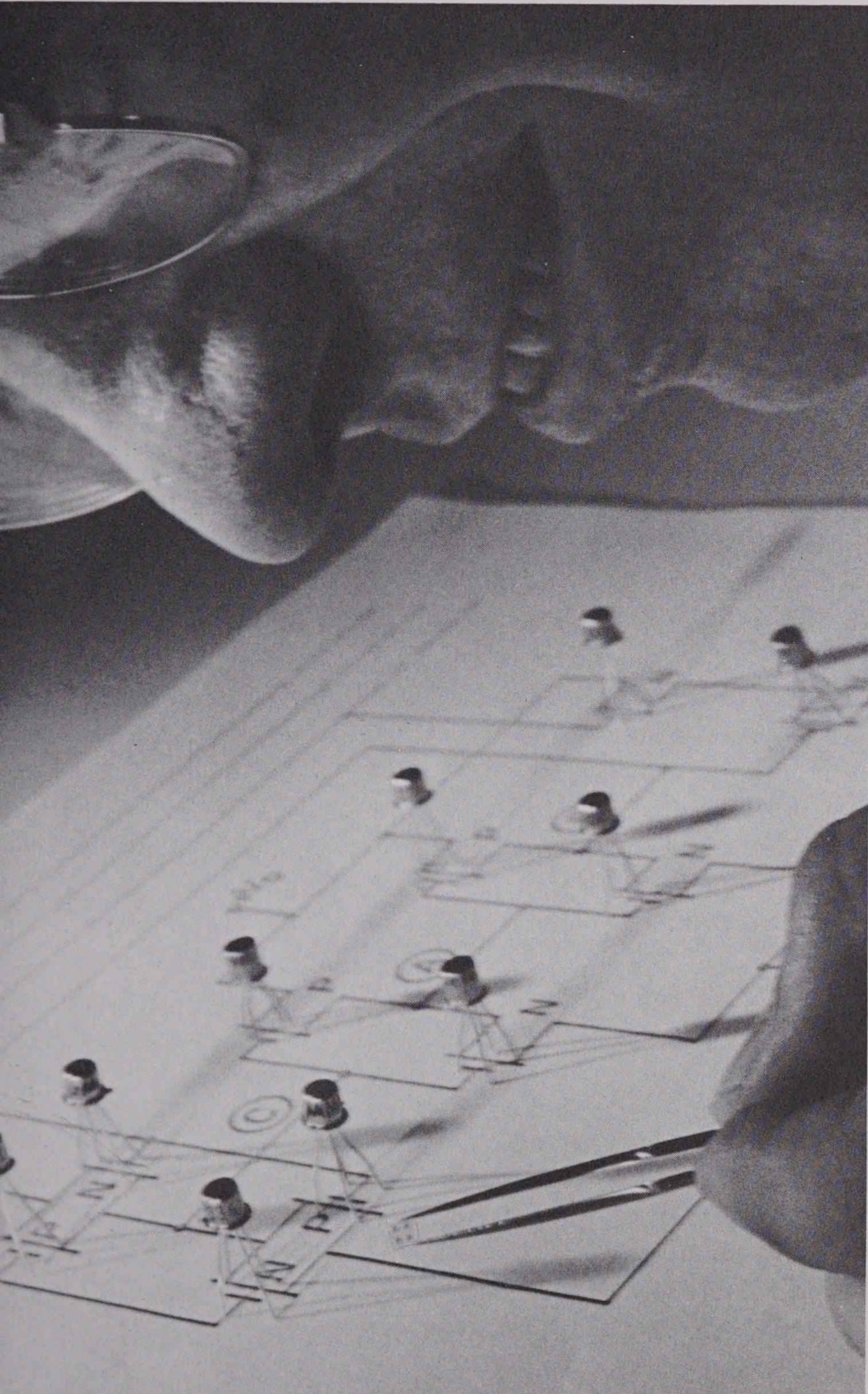
A conventional transistorized circuit is compared by Dr. Charles Mueller with four silicon-on-sapphire thin-film circuits, each of which is the electronic equivalent of the conventional circuit.
