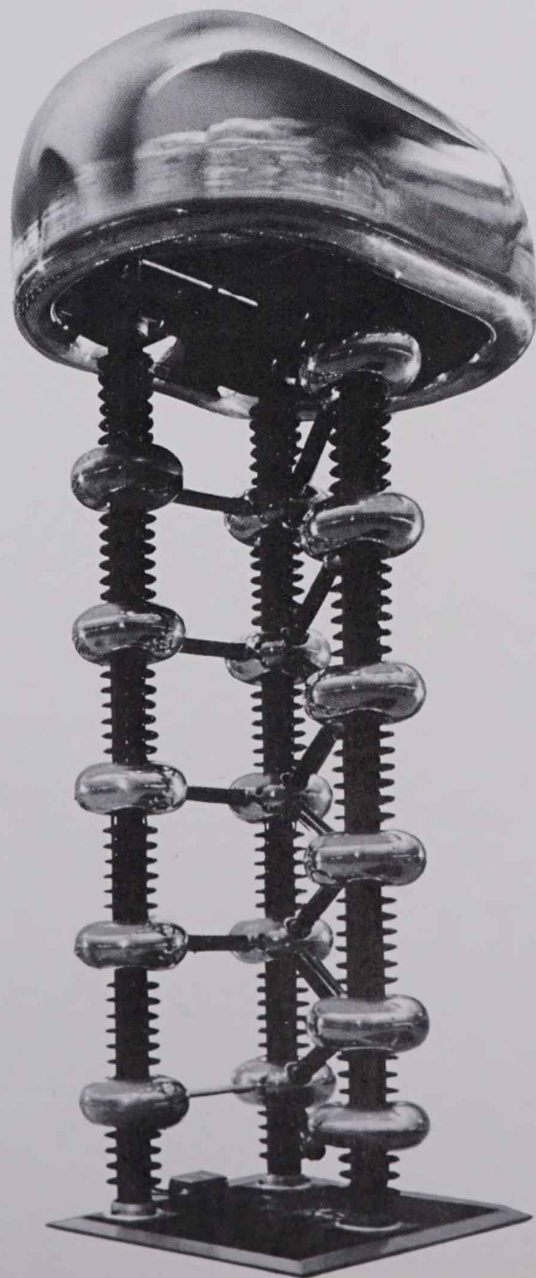
Accelerator for million-volt electron microscope at U.S. Steel Corporation
