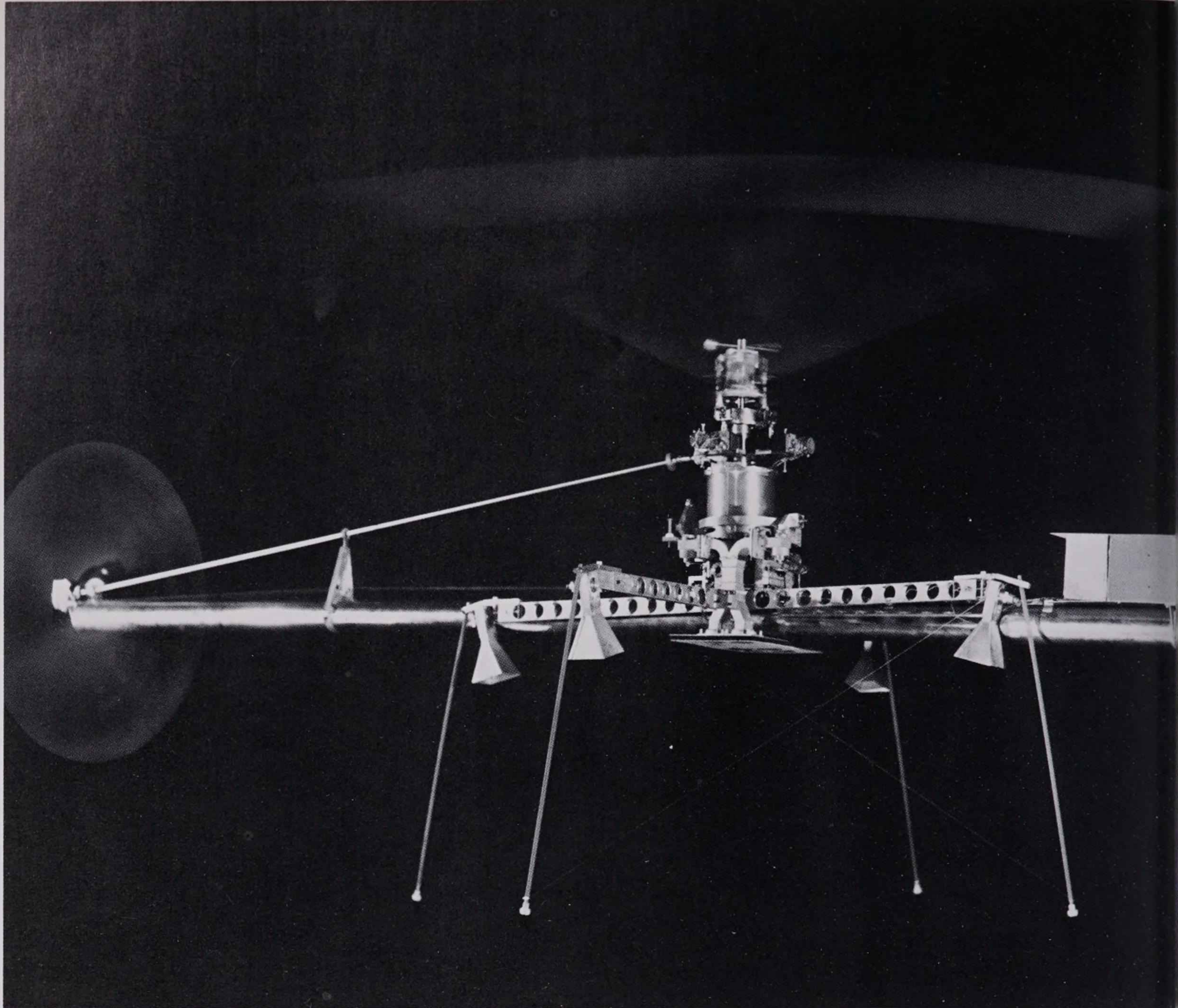
Microwave power lifts this pilotless helicopter 50 feet into the air.
