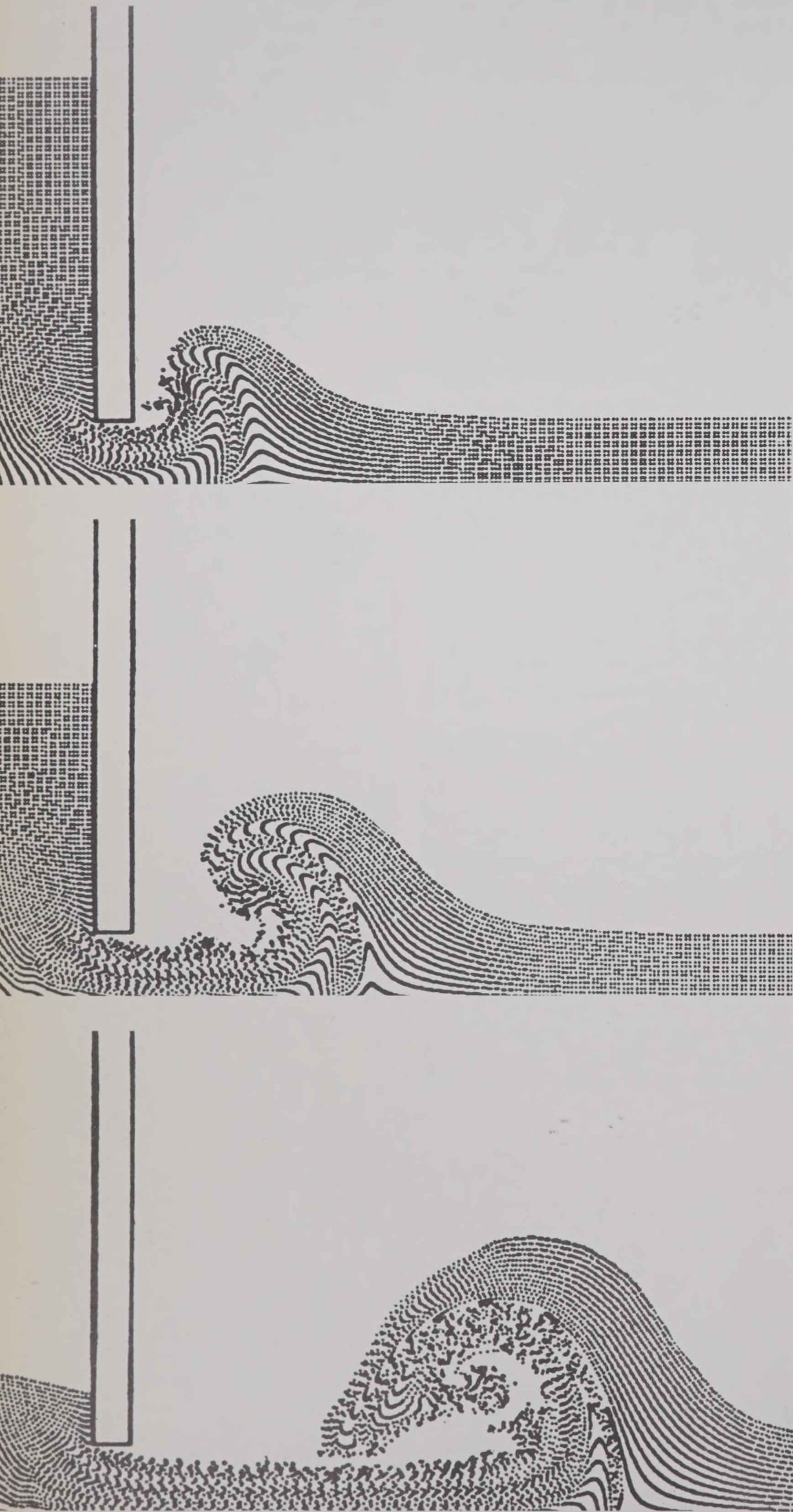
Frames of a computer-produced film depict the escape of water under a gate.
