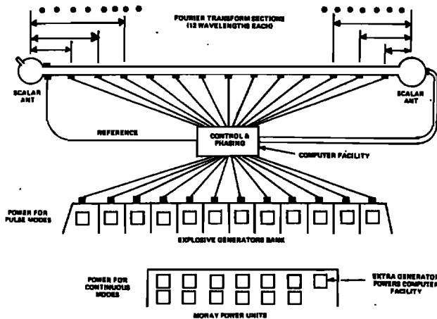
Item 1. TESLA WEAPON AT SARYSHAGAN (SCALAR POTENTIAL INTERFEROMETER)
