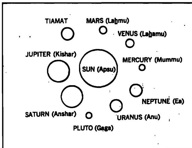
Fig. 3 - Related celestial etymological names.
