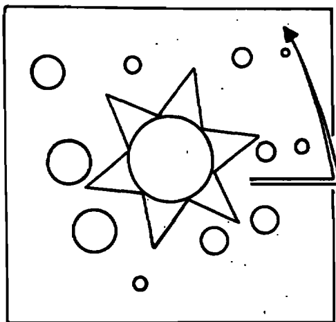
Fig. 2 - Enlargement of Sumerian celestial map.
