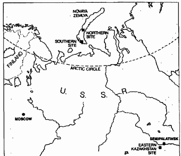
Soviet nuclear test sites at Novaya Zemlya and Semipalatinsk.
