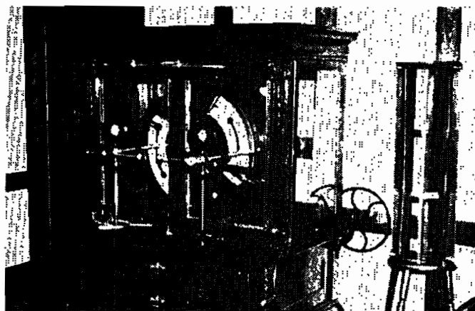
Large-cased Holtz-Toepler generator of U.S. manufacture (c. 1900), retrieved from Mexico. Used to power X-ray. An air-core high-frequency solenoid, also from c. 1900, on the right.
