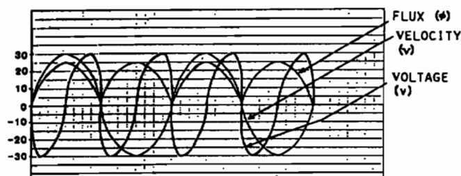
TWO CYCLES OF FLUX AND VELOCITY AND THE RESULTING FOUR CYCLES OF VOLTAGE IN THE DYNAFLUX GENERATOR
