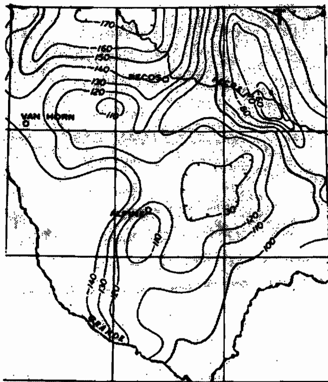
Figure B Gravity Anomaly Map
