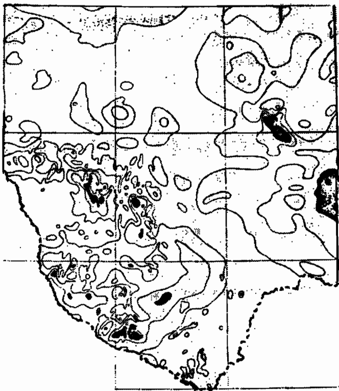
Figure A Magnetic Anomaly Map
