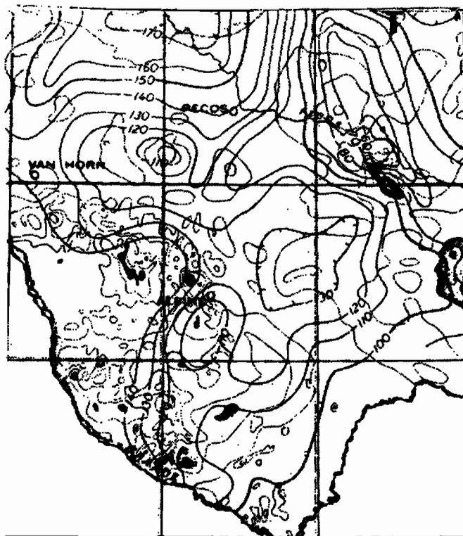
Figure C (Figures A & B Superimposed)
