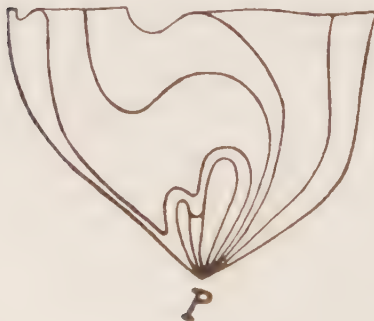
Fig. 5. Parabolic sector.
