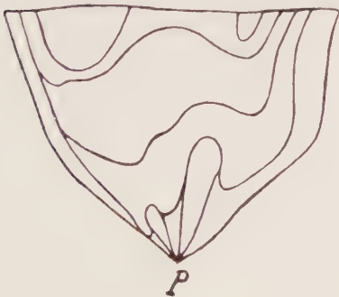
Fig. 3. Hyperbolic sector.
