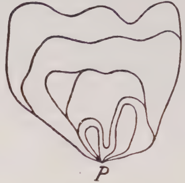
Fig. 4. Elliptic sector.
