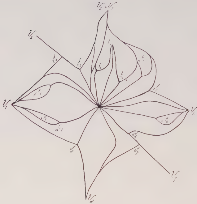
Fig. 1. Irrigation territory.
