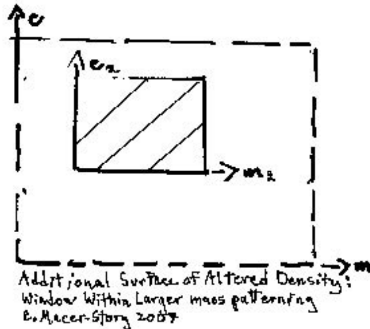
Figure seven: additional surface within locally coherent e/m mass density
