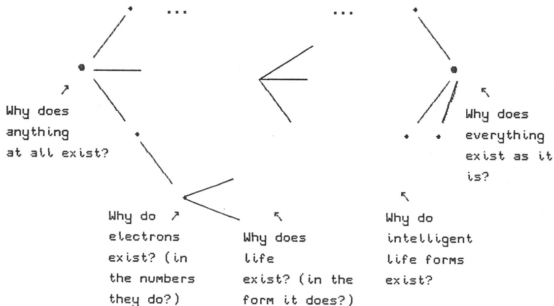
DIAGRAM 2. (Bounded) lattice of questions. 3
