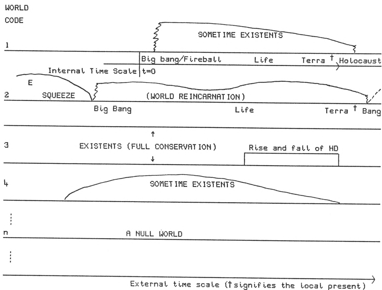
DIAGRAM 4. Dynamic picture of worlds modelling of theme C), with sample universes.
