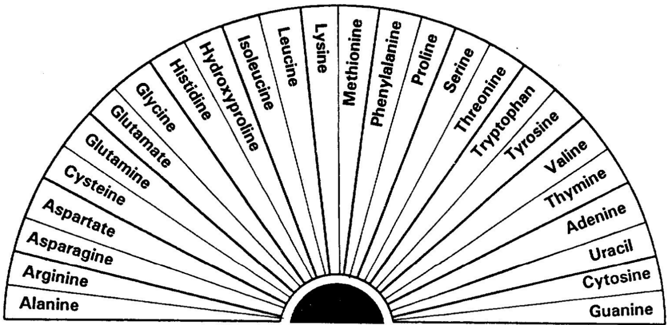
Amino Acids
