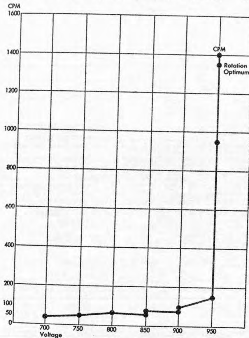
Chart D. CONTROL TUBE (1), kept OUTSIDE OR laboratory, after one month exposure to OR energy field of OR room, 100 ft. distance, has soaked up enough OR energy to yield rotary motor effect; measured during eleven consecutive minutes (Sept. 29, 1947).
