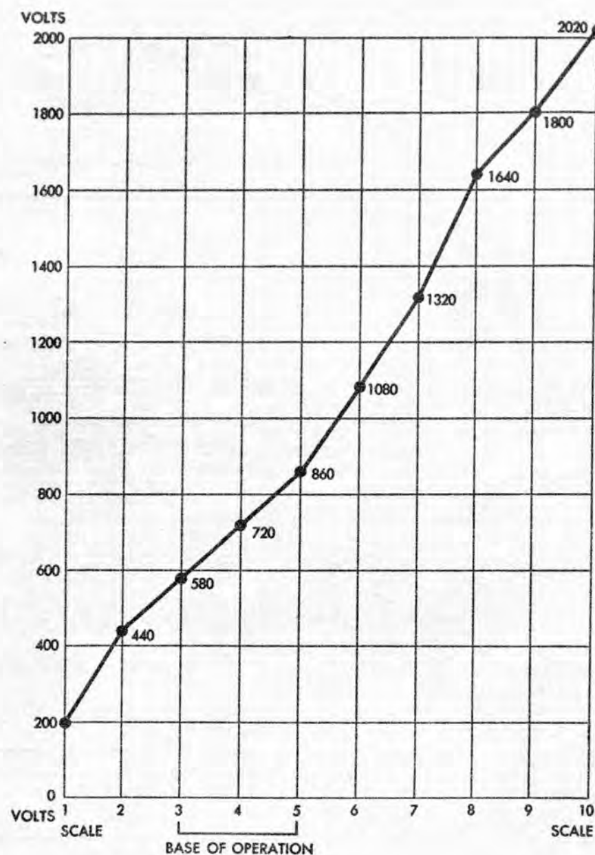
Chart E. Calibration of electroscope, aluminum leaf. 1 ORG = 256 Volts.
