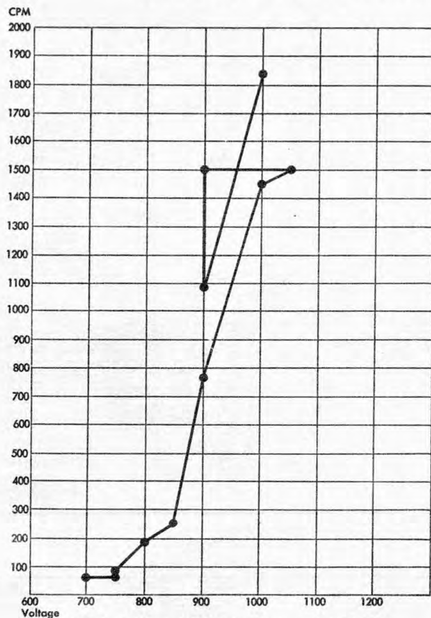
Chart A. CPM with GM Counter CMB-3A, Tube GLC-II, Aug. 31, 1947, 2:30-3 P.M.
