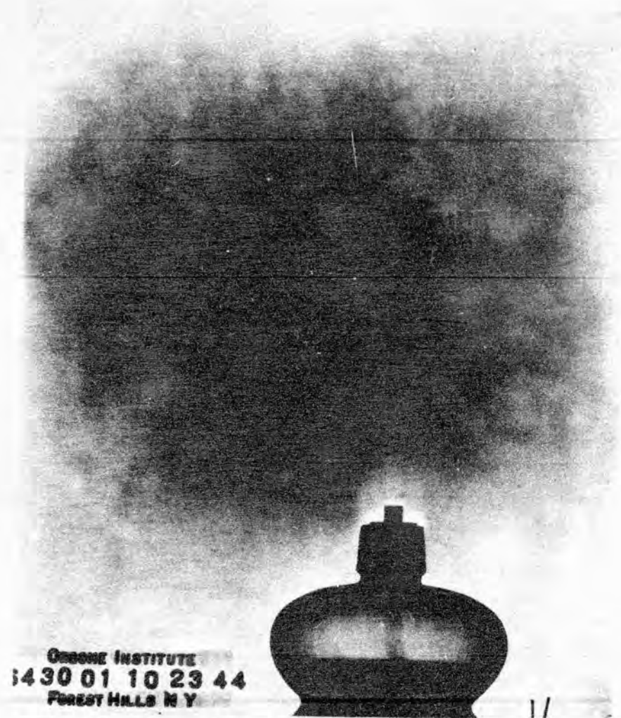
Photo 3. Xray photograph of OR energy field from an alcohol flame. The flame was placed between the Xray tube and the Xray plate. Exposure: 0.1 second, 64 kv, 30 ma.
