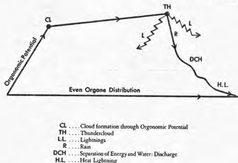
Fig. 1. Charge and Discharge in Thunderstorm
