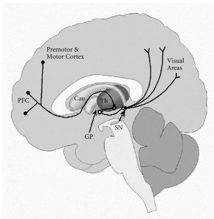
Figure 5. A procedural-memory-based category learning system. Excitatory projections end in solid circles, inhibitory projections end in open circles, and dopaminergic projections are dashed. PFC = prefrontal cortex, Cau = caudate nucleus, GP = globus pallidus, and Th = Thalamus.
