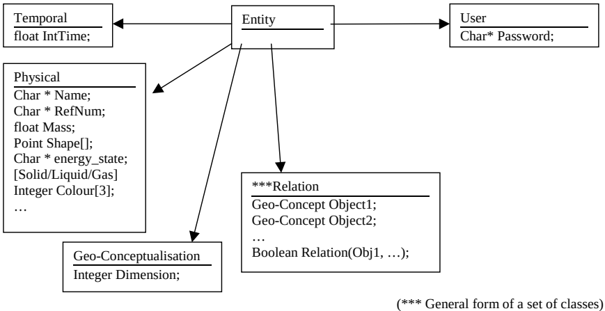
Figure 5. Base classes (Abstract)
