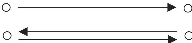
Figure 1a,b. Direct path and symmetry of path relation
