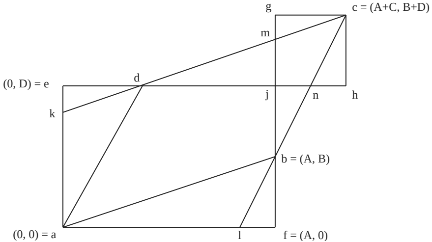
Figure 1. A 2 \times 2 Determinant is the Area of a Parallelogram after Nelson (1993: 133)
