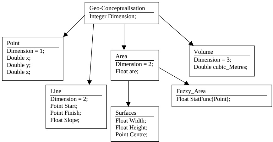
Figure 6. The Geometric Conceptualisation classes
